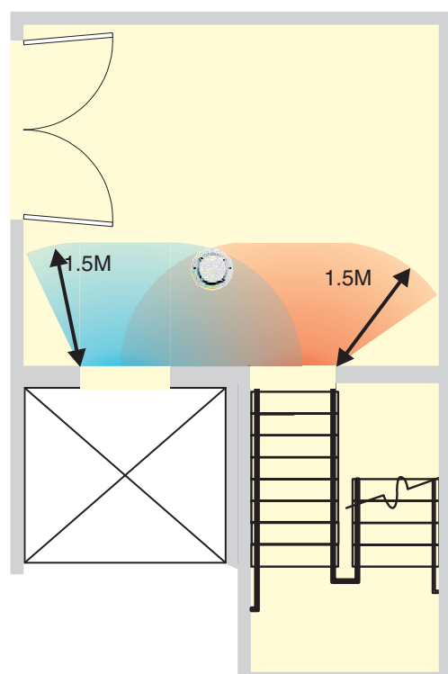
Figure 27: Protection of vertical shafts
